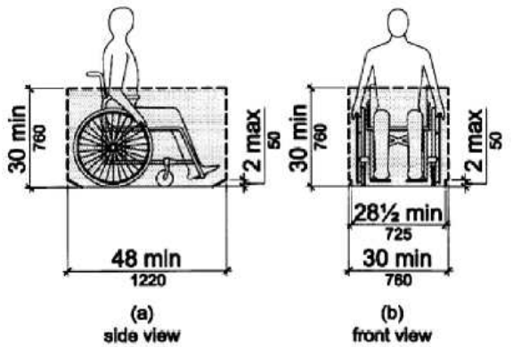
Figure 1 Wheelchair or Mobility Aid Envelope
