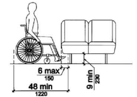
Figure 2 Toe Clearance Under a Fixed Element
