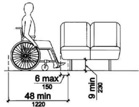
Figure 2 Toe Clearance Under a Fixed Element
