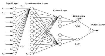
Fig. 3. The modified PNN for a two-class classification problem (Abdullah and Ritchie, 1999).
