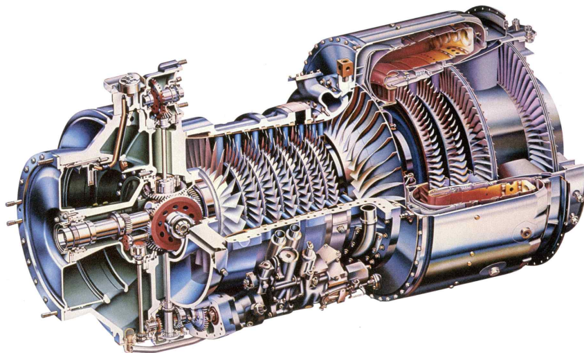
T55 TURBOSHAFT ENGINE ALLIED SIGNAL ENGINES
